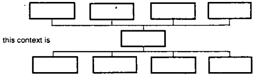
STRATIGRAPHIC MATRIX
