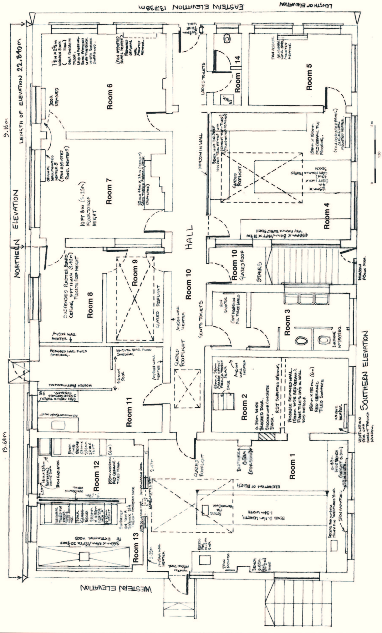
Figure 3: Laboratory floor plan (Building no. 14)
