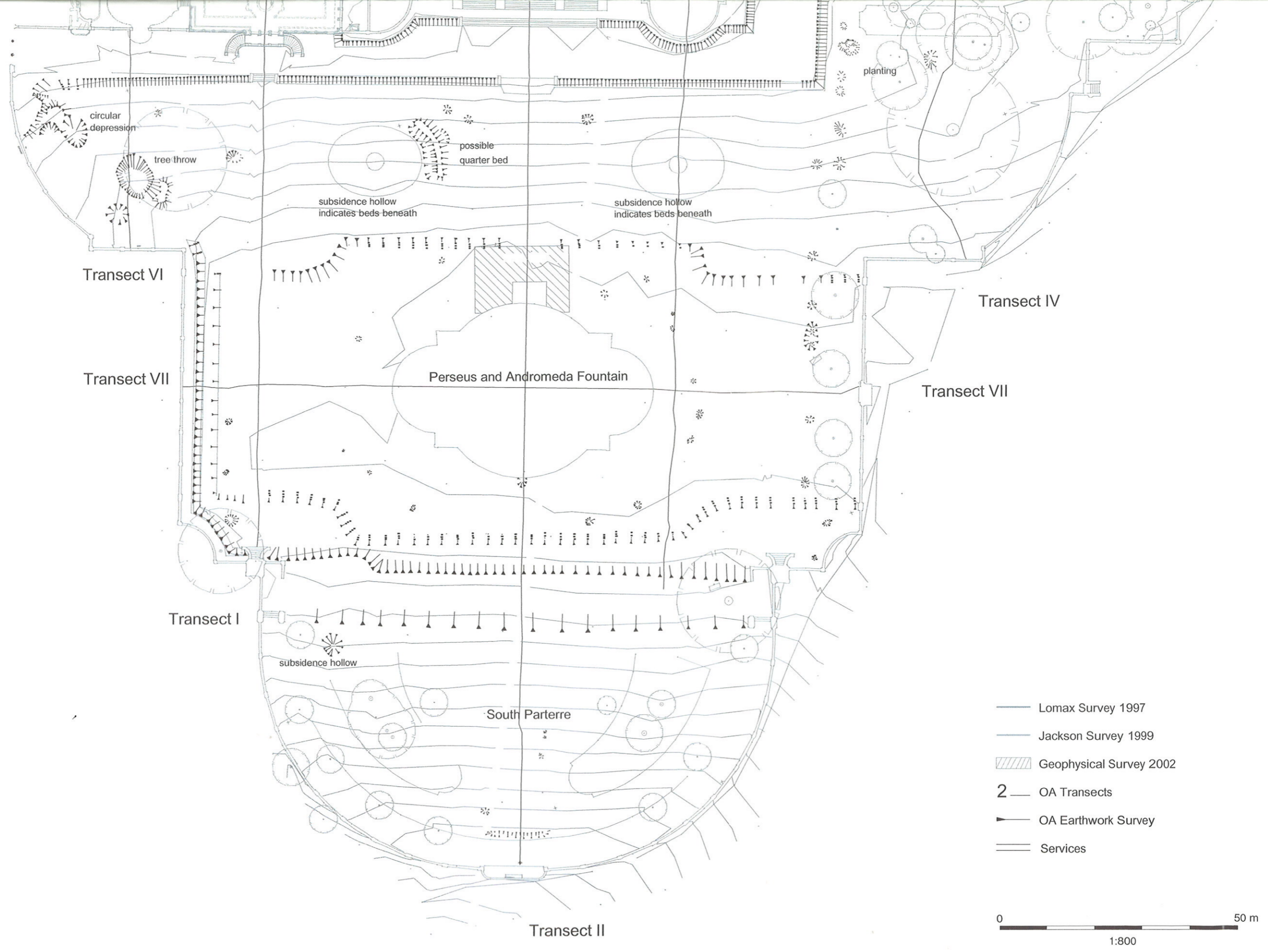
Figure 2 : Topographical Survey of the Gardens
