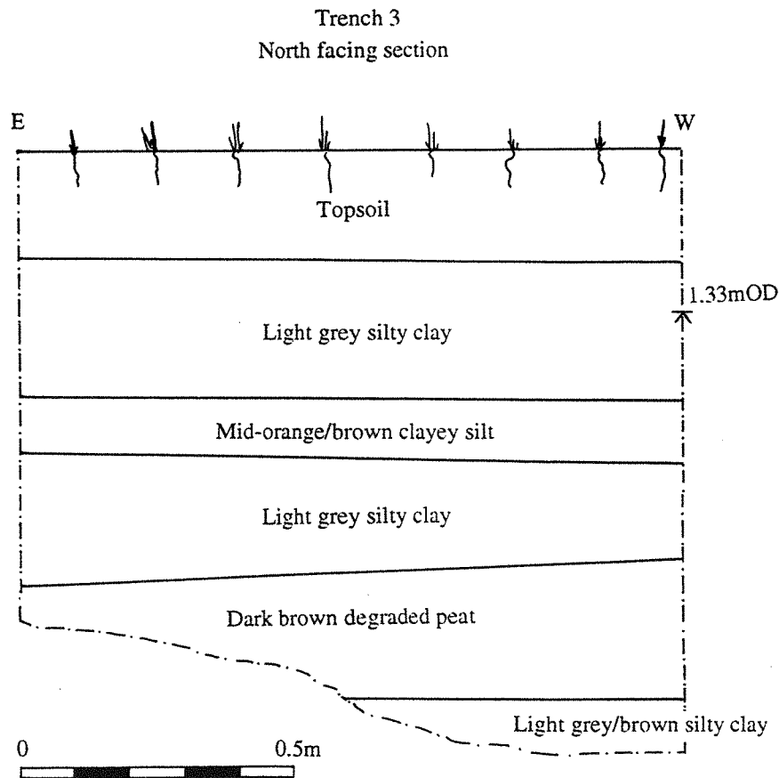
Figure 2 Schematic section of site stratigraphy
