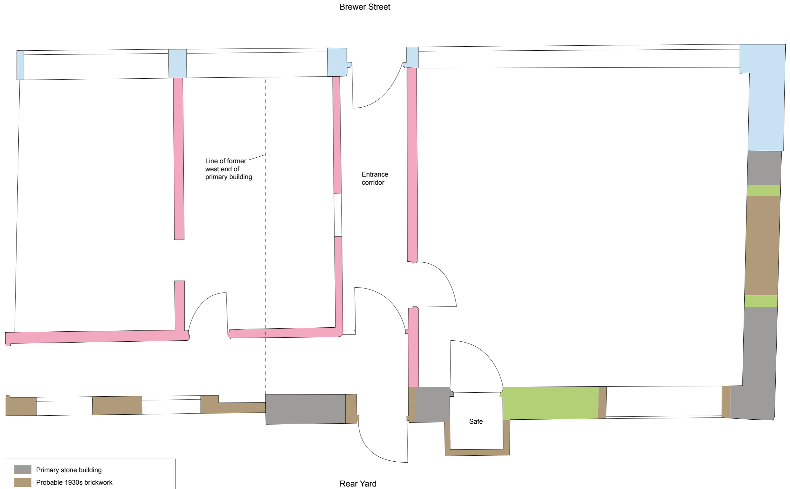
Figure 7: Ground floor plan of 6 Brewer Street 6 Brewer Street, Oxford and associated structures Oxford Archaeology
