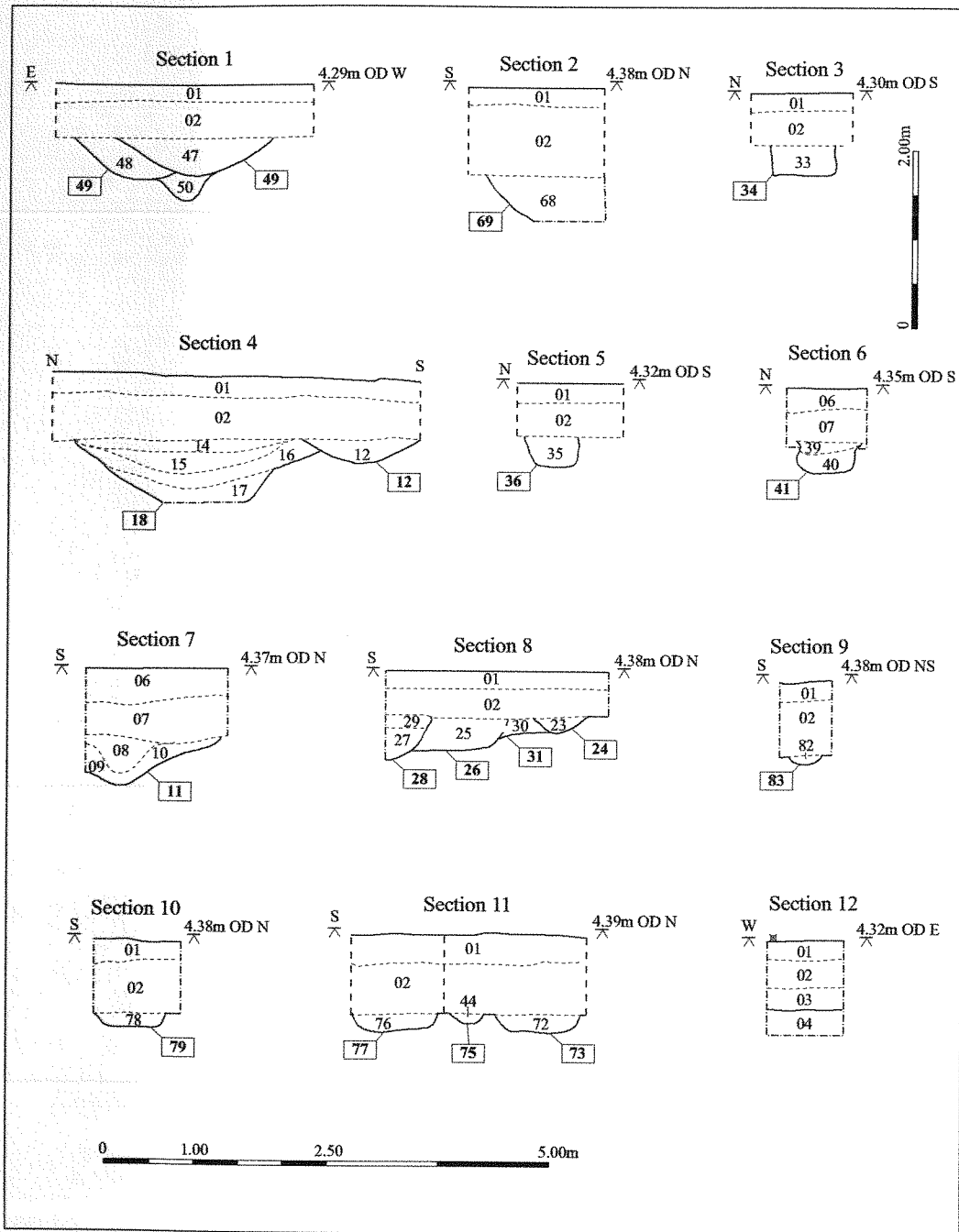
Figure 3 Trench Plans
