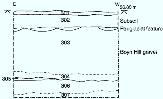
Test Pit 3 Section
