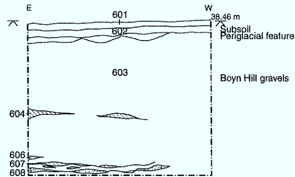
Test Pit 6 Section
