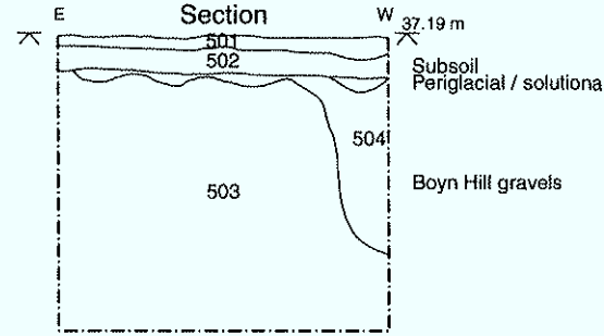
Test Pit 5 Section
