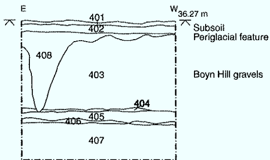
Test Pit 4 Section
