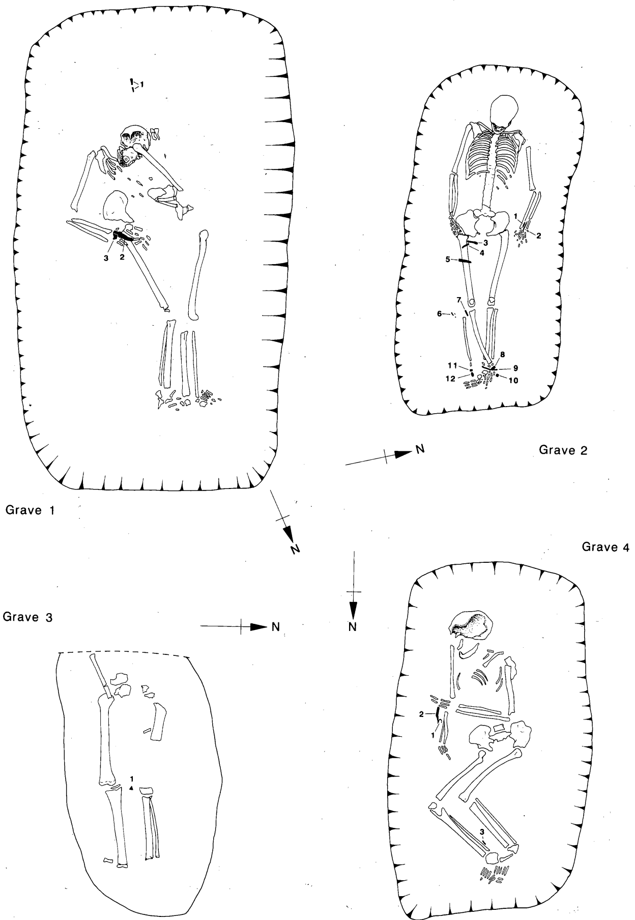
Figure 90 Grave plans 1-4
