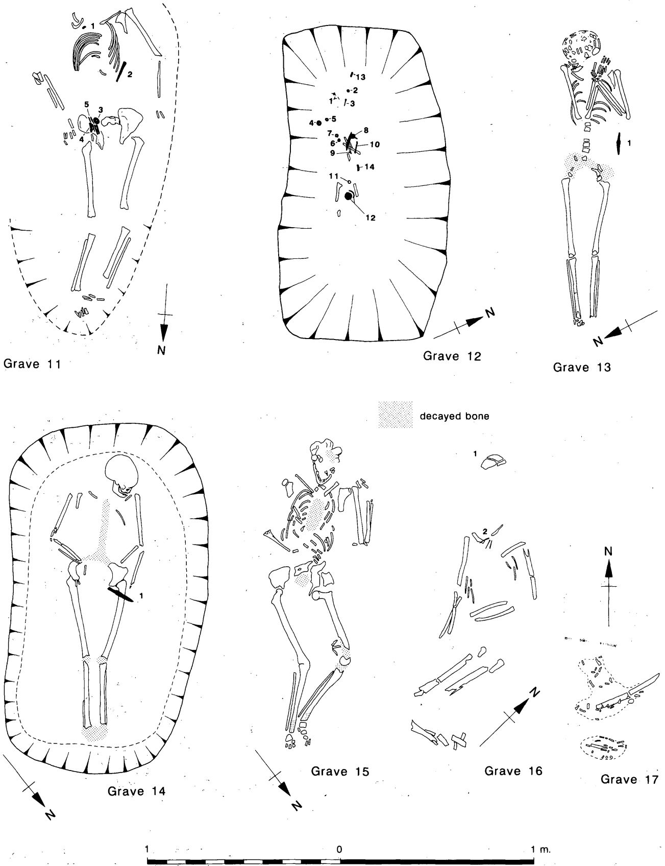
Figure 92 Grave plans 11-17
