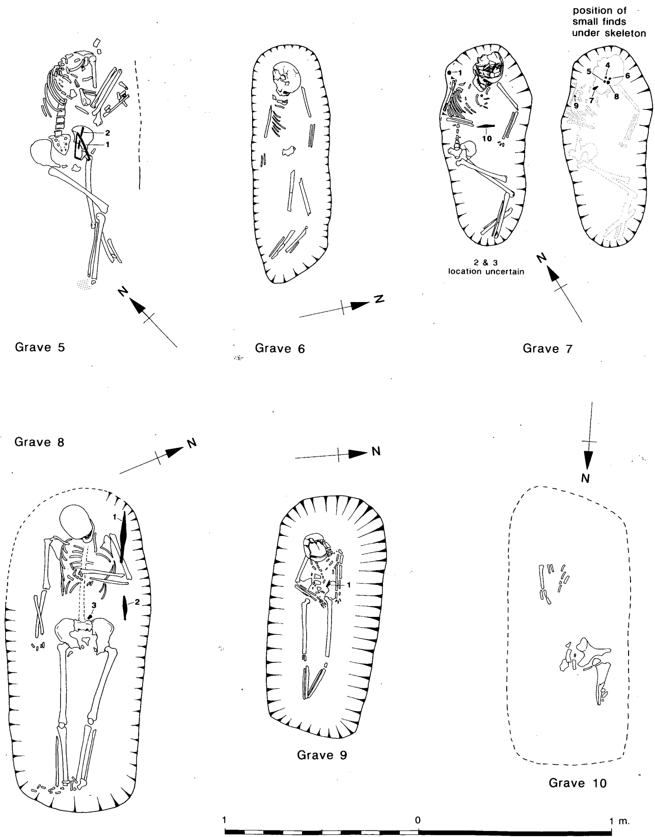
Figure 91 Grave plans 5-10
