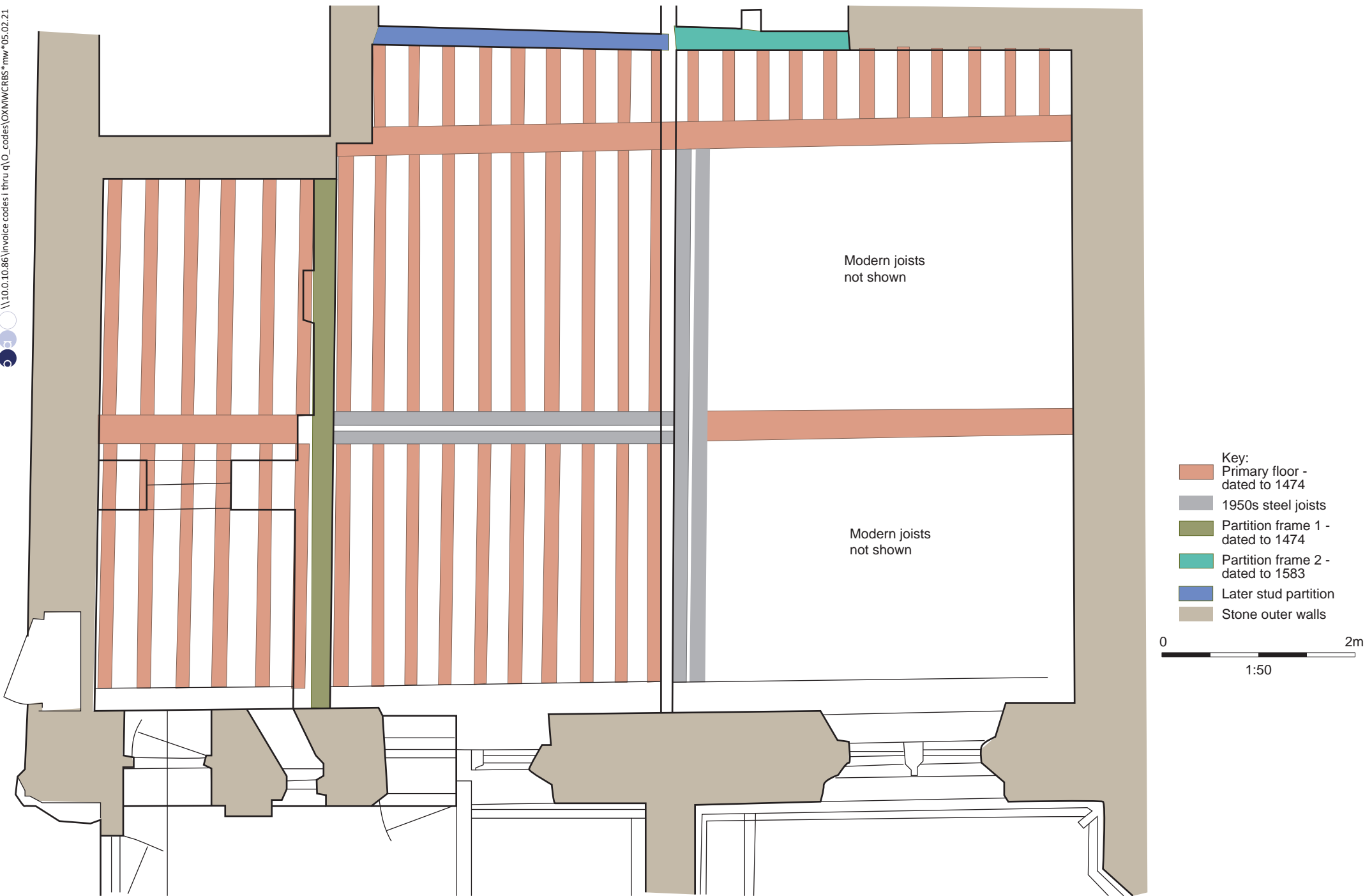
Figure 11: Plan of floor joists in Old Bursary area
