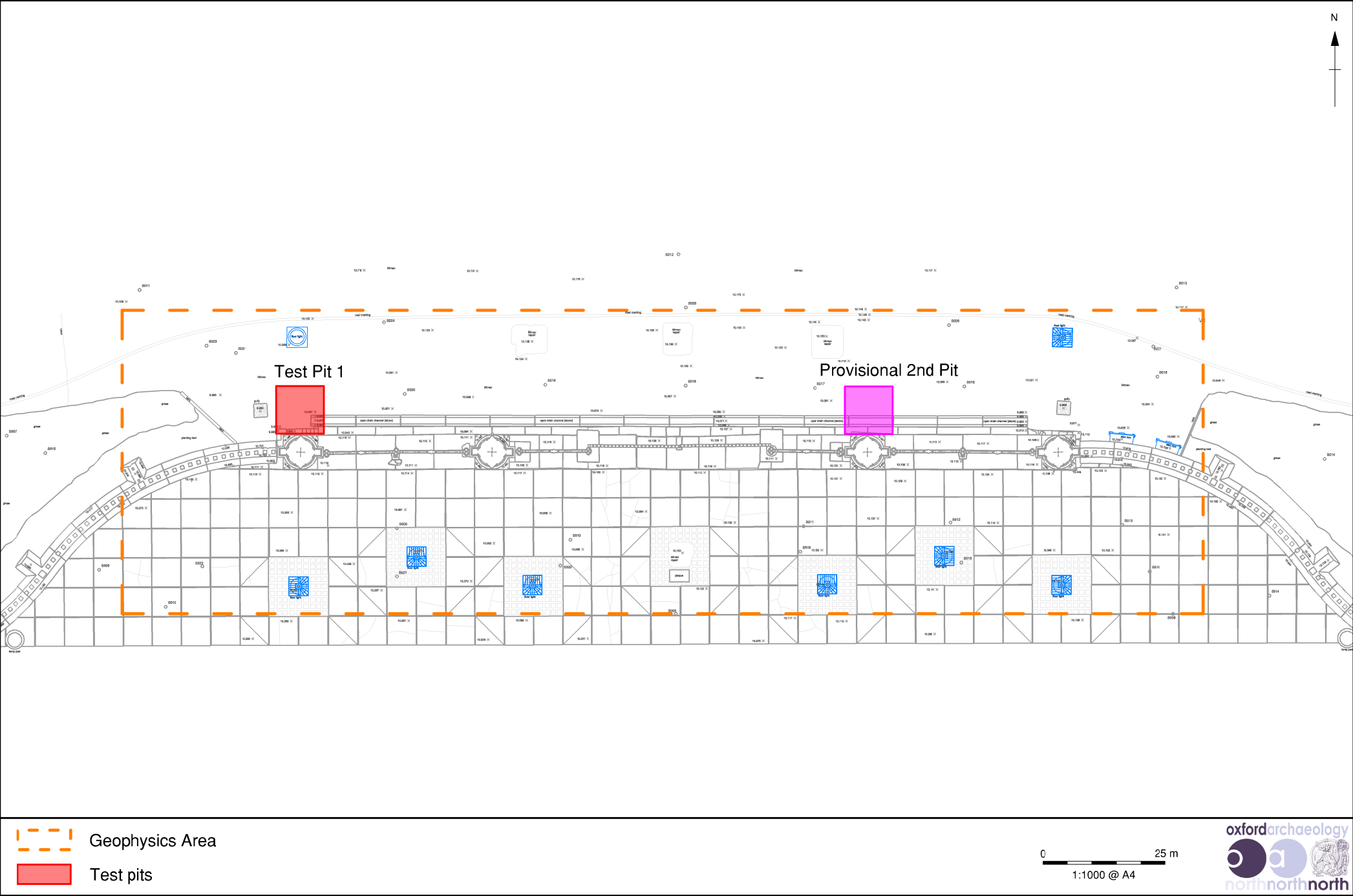
Figure 2: Site plan
