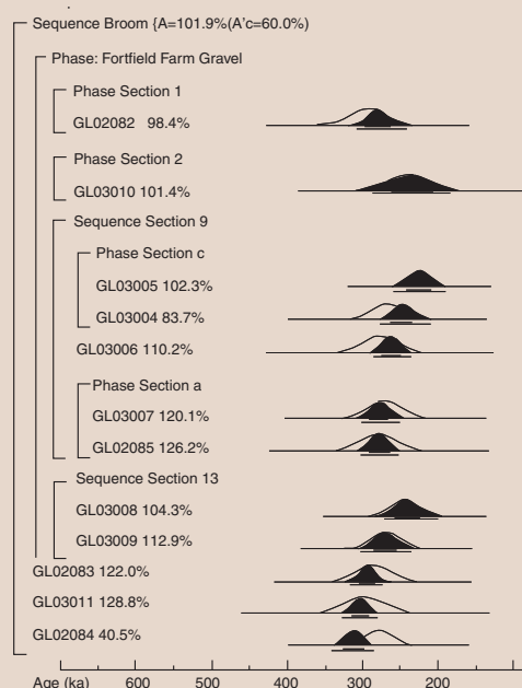
2.5.3 Bayesian modelling of accepted optical age estimates within the Broom Sand and Silt Bed (from Hosfield et al. 2011)
