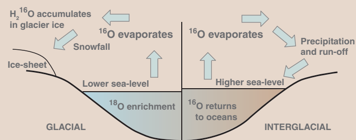
2.1.2 Effects of glacial and interglacial periods on the ^{18}\text{O}/^{16}\text{O} ratio of sea water
