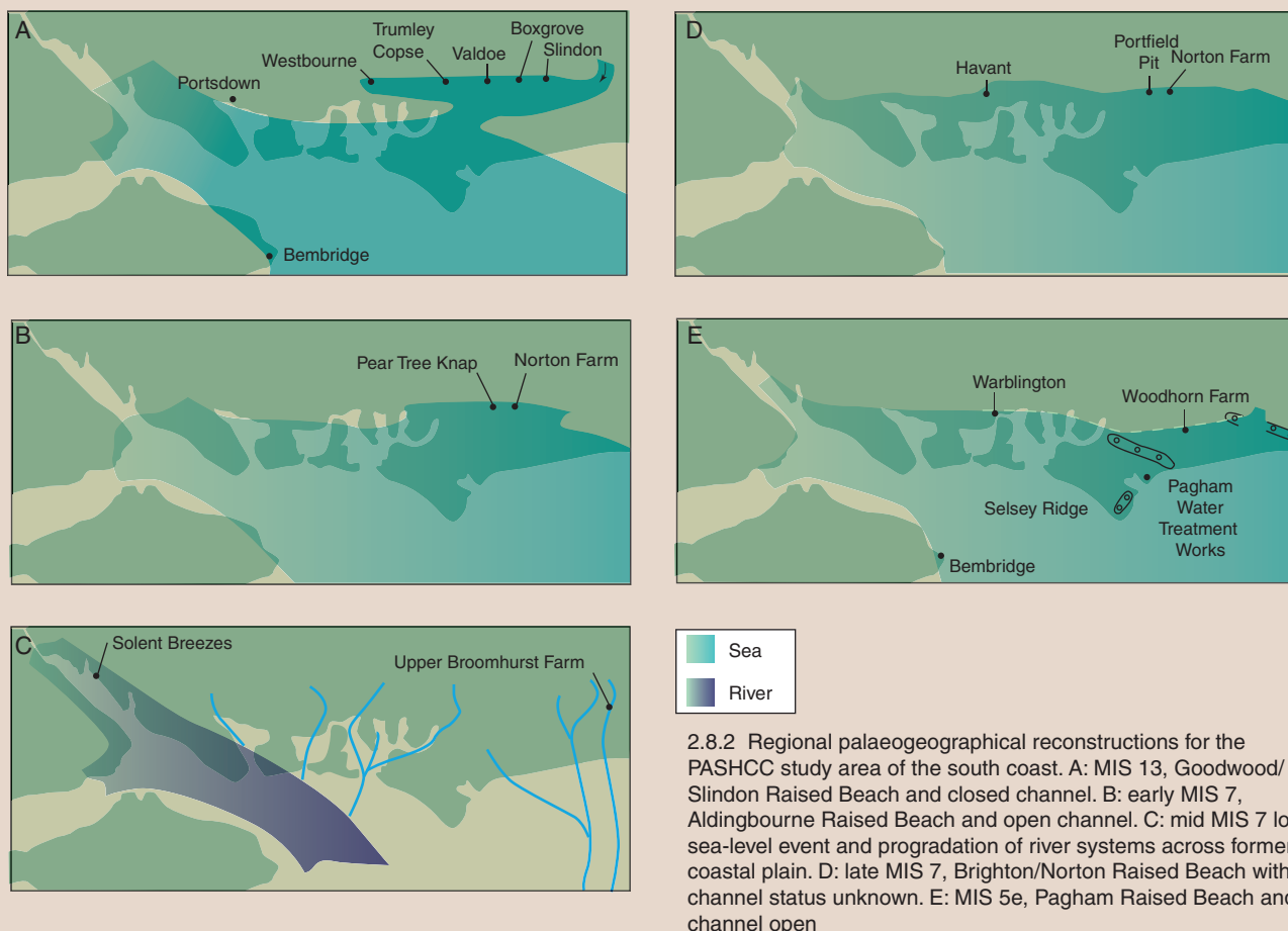
2.8.1 OSL dates from the West Sussex Coastal Plain area plotted against Marine Isotope Stages
