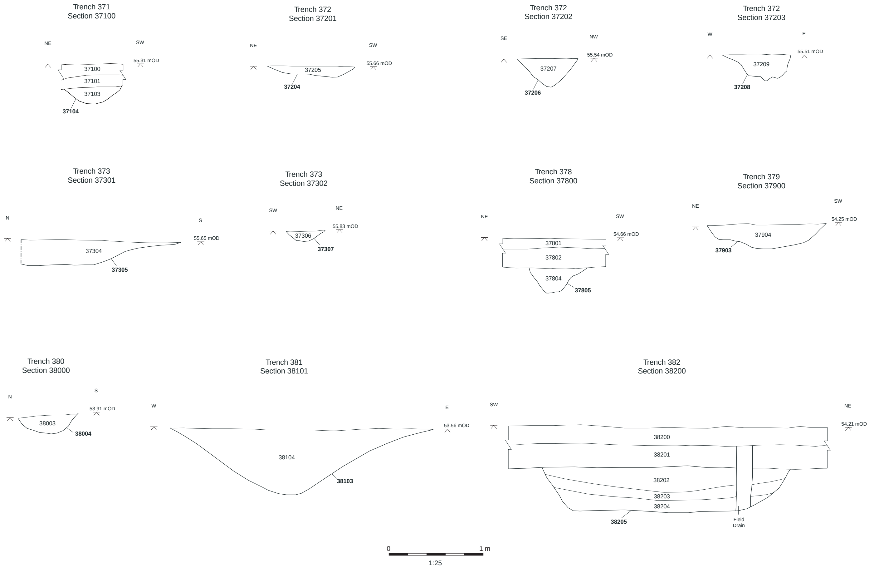
Figure 32: Areas 1 and 2, selected sections, Trenches 371, 372, 373, 378, 379, 380, 381, 382
