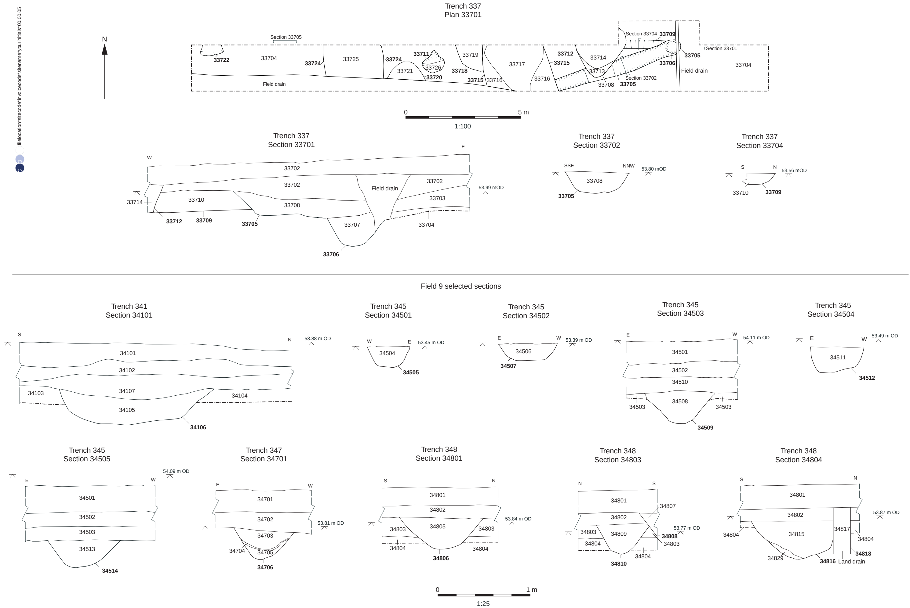
Figure 31: Field 9, Trench 337 plan and selected sections, Trenches 341, 345, 347, 348 selected sections
