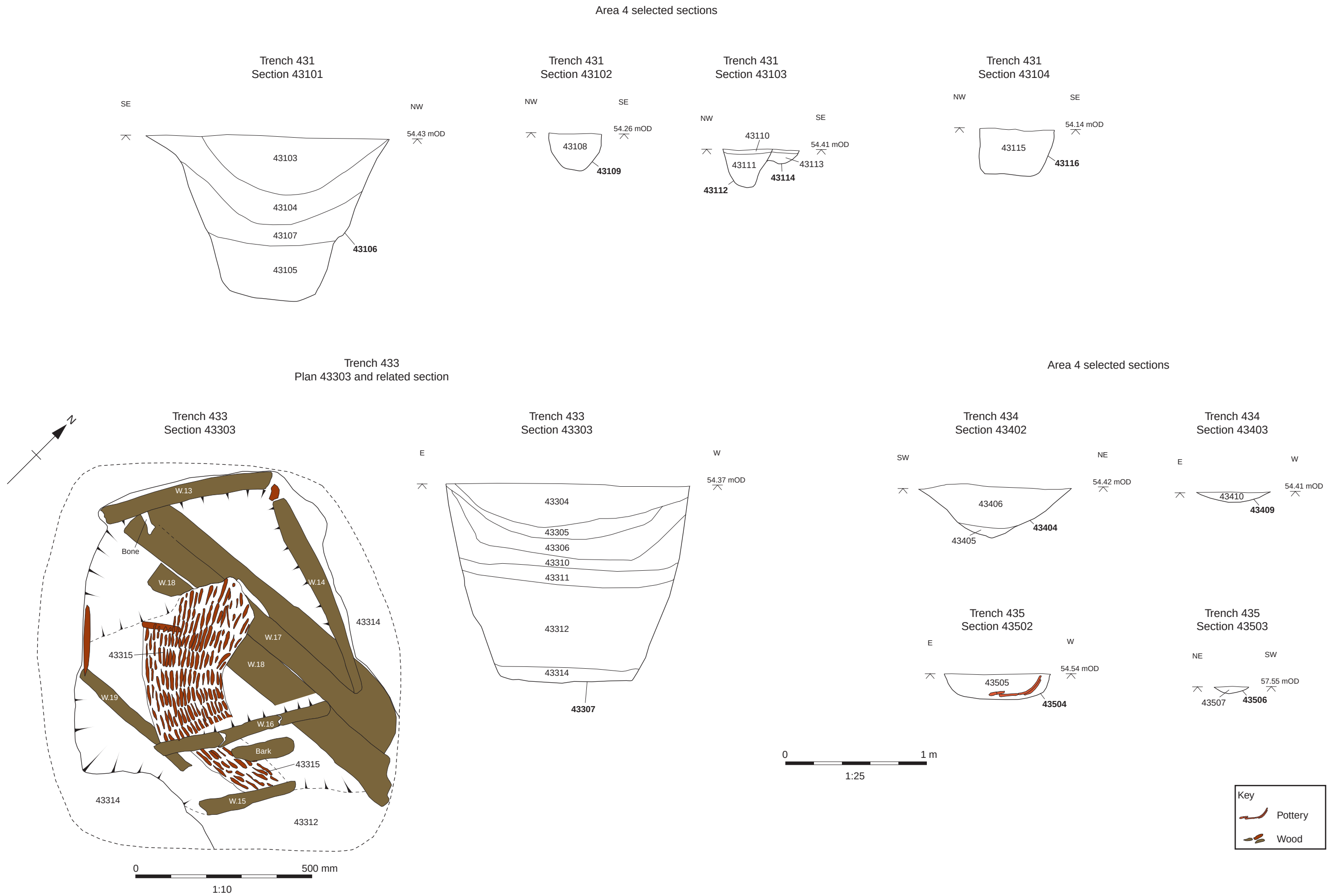
Figure 43: Area 4, Trench 433 plan and selected sections, Trenches 431, 434, 435 selected sections
