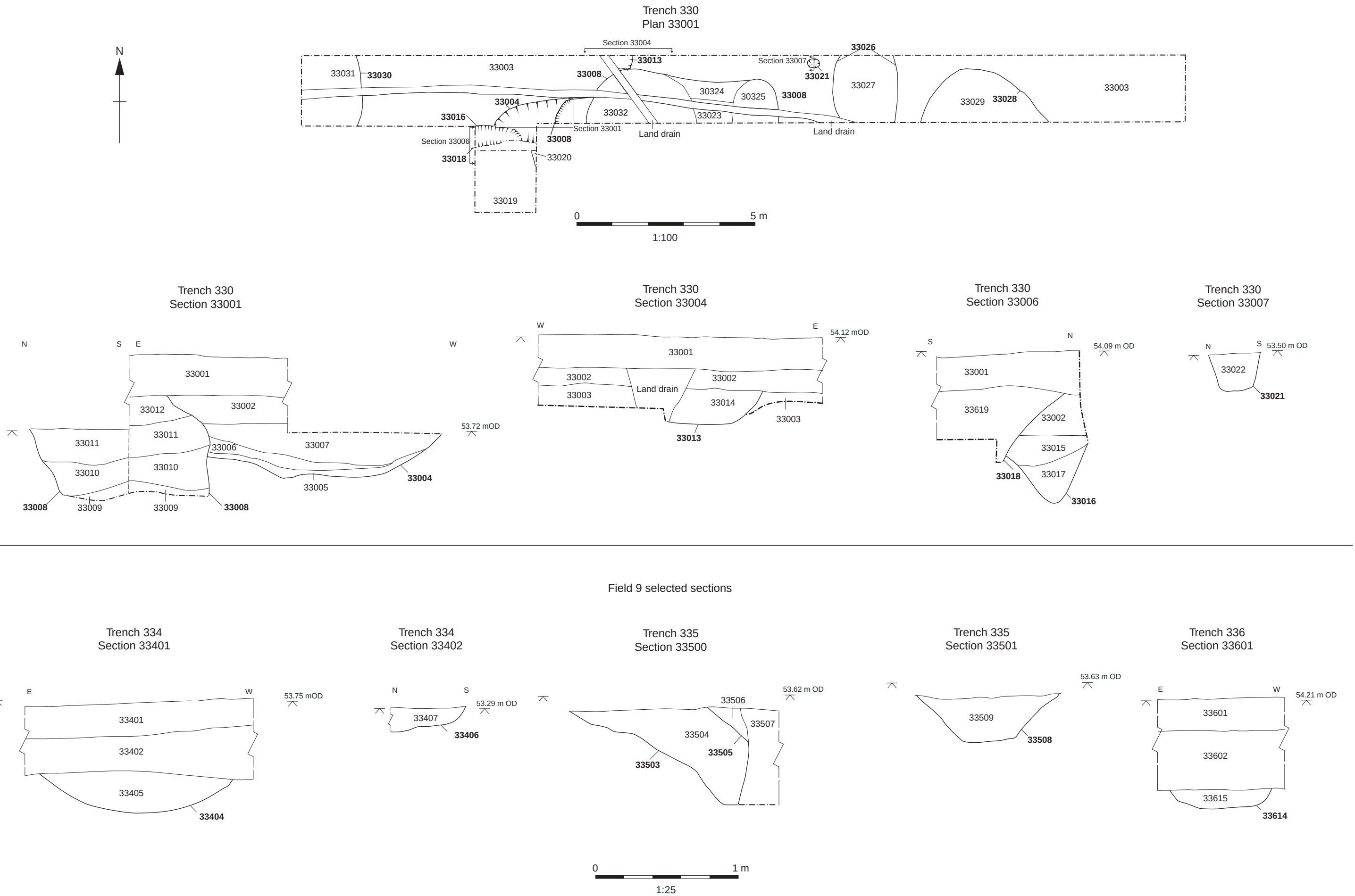
Figure 30: Field 9, Trench 330 plan and selected sections, Trenches 334, 335, 336 selected sections
