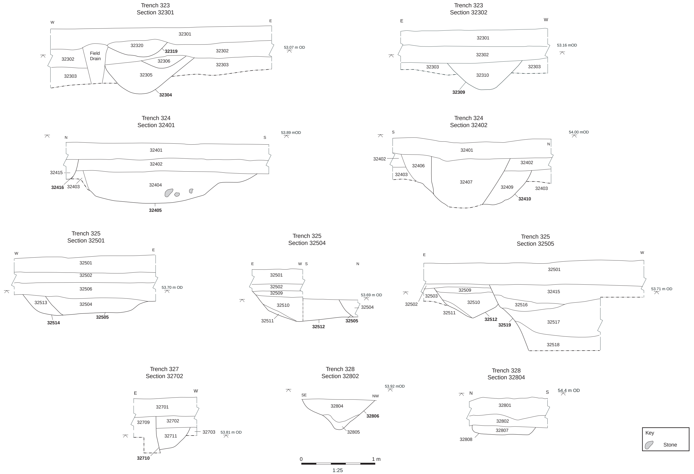
Figure 29: Field 9, selected sections, Trenches 323, 324, 325, 327, 328
