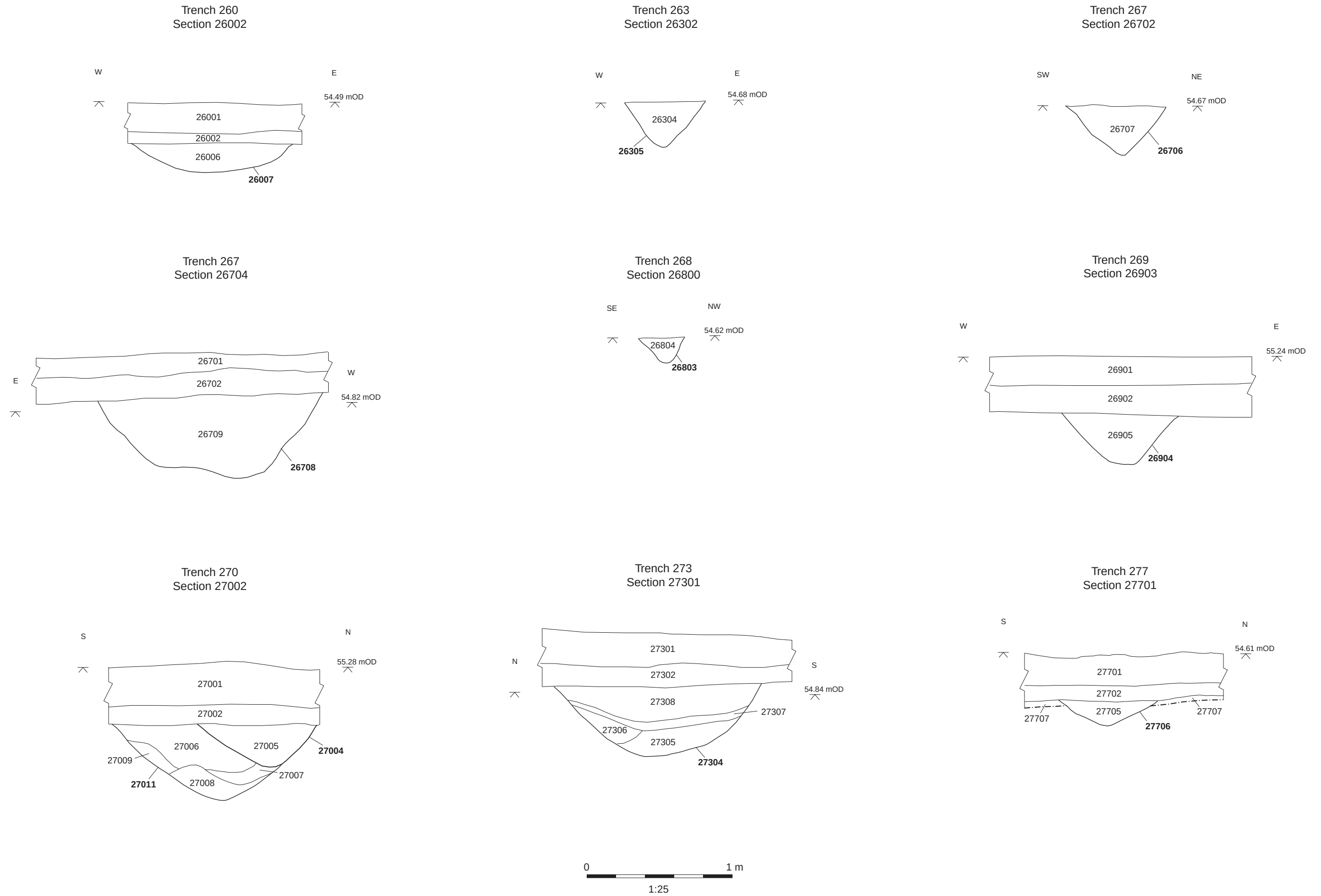
Figure 26 : Field 6, selected sections, Trenches 260, 263, 267, 268, 269, 270, 273 and 277
