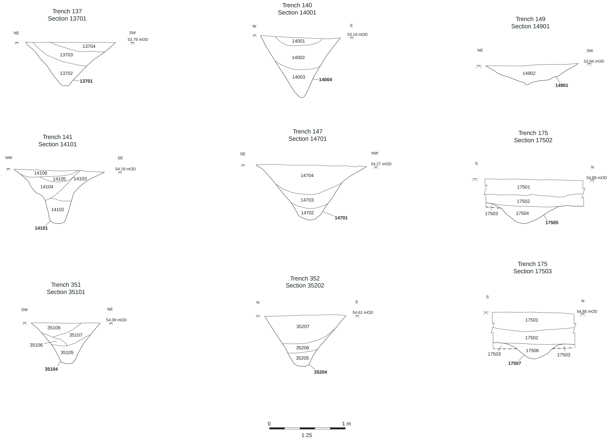
Figure 18: Fields 1 and 2, selected sections, Trenches 137, 140, 141, 147, 149, 175, 351, 352
