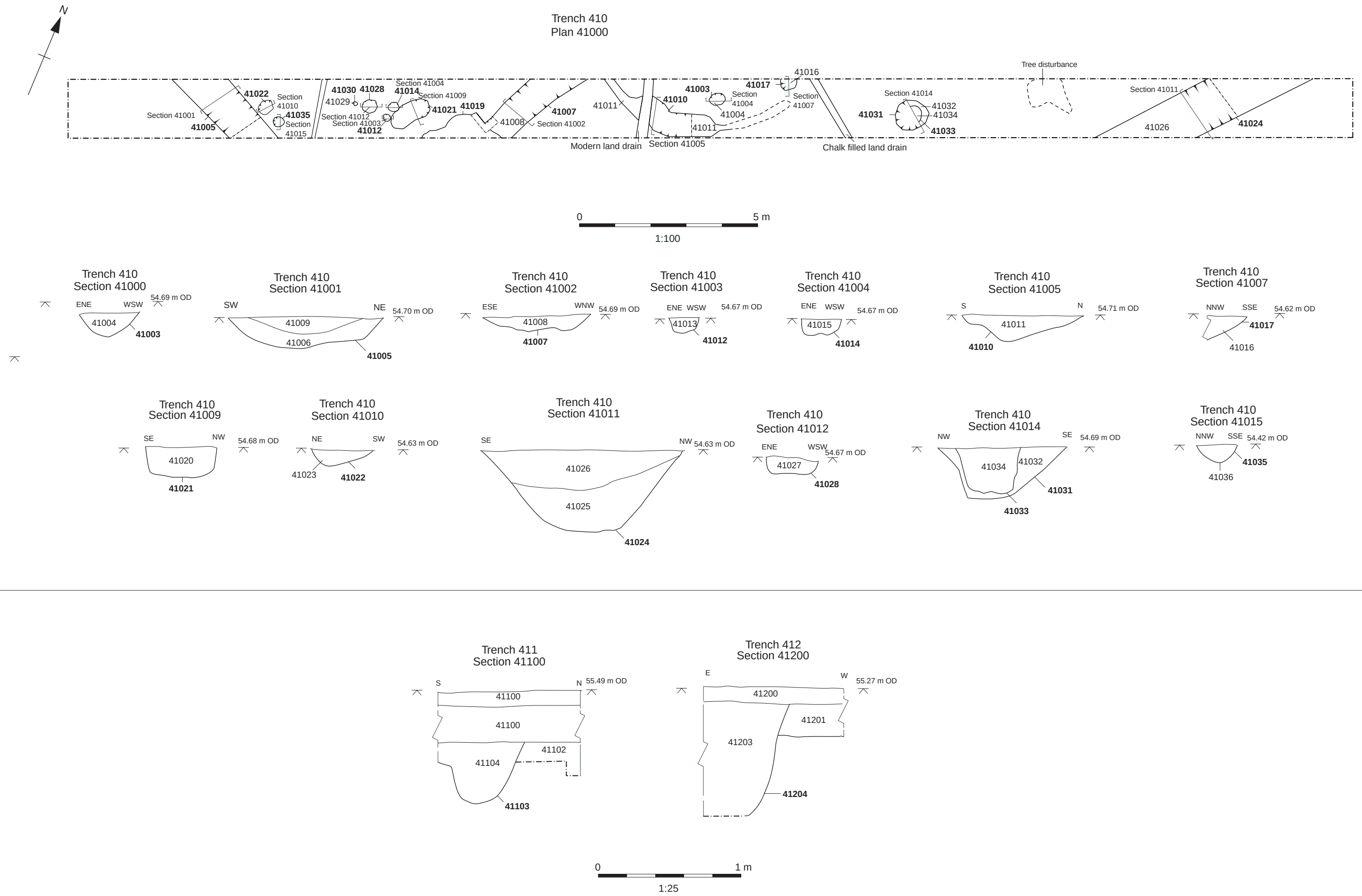
Figure 39: Area 3, Trench 410 plan and sections, Test pits 411 and 412 sections
