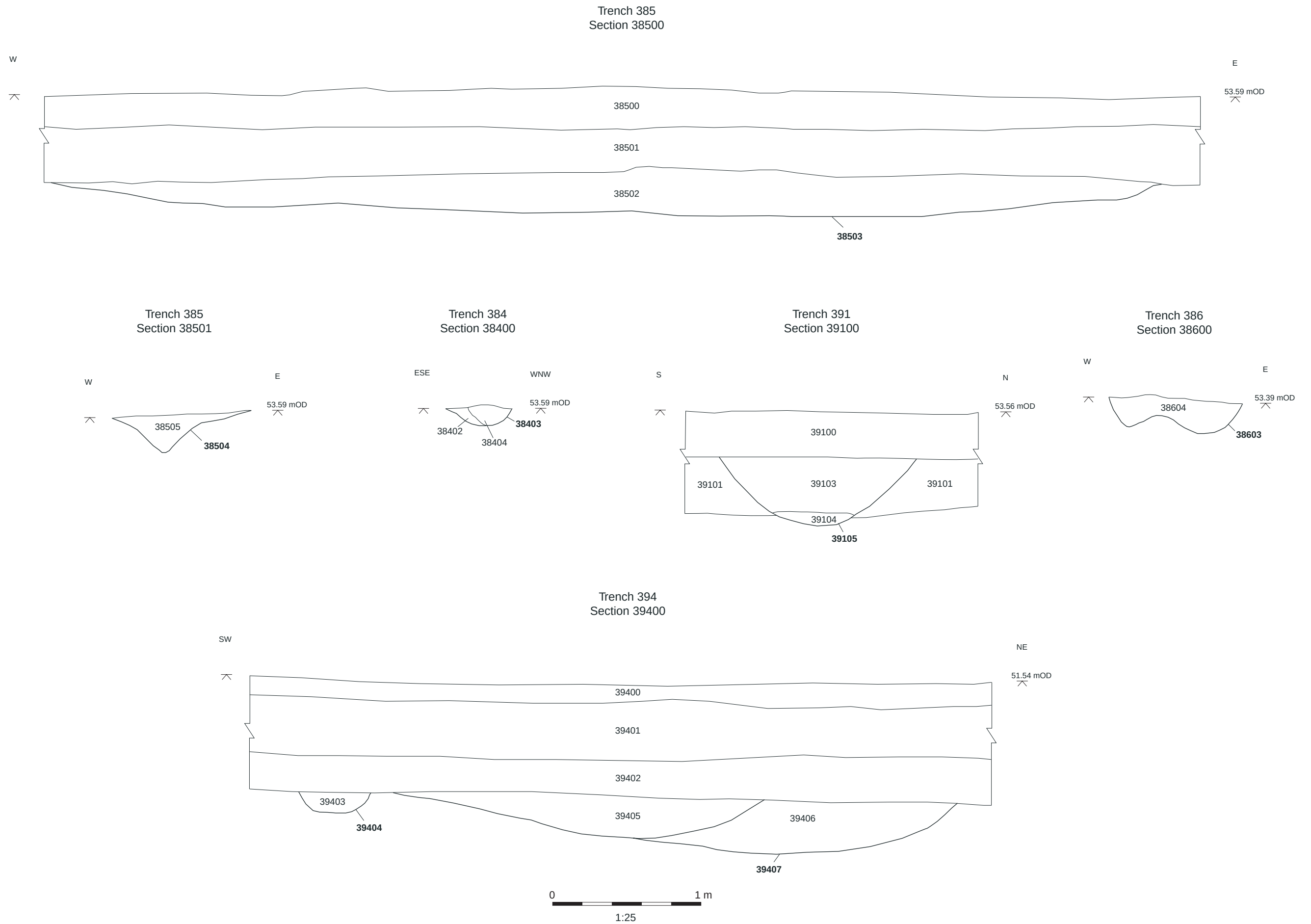
Figure 33: Areas 1 and 2, selected sections, Trenches 384, 385, 386, 391, 394
