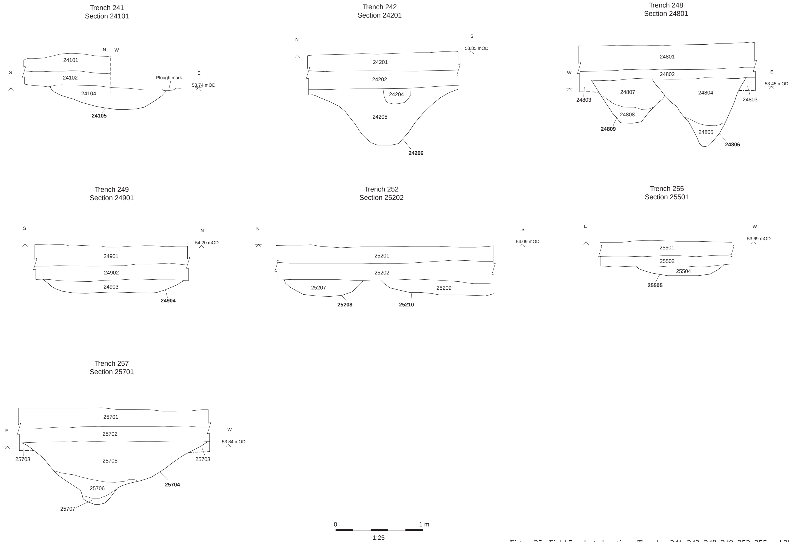
Figure 25: Field 5, selected sections, Trenches 241, 242, 248, 249, 252, 255 and 257
