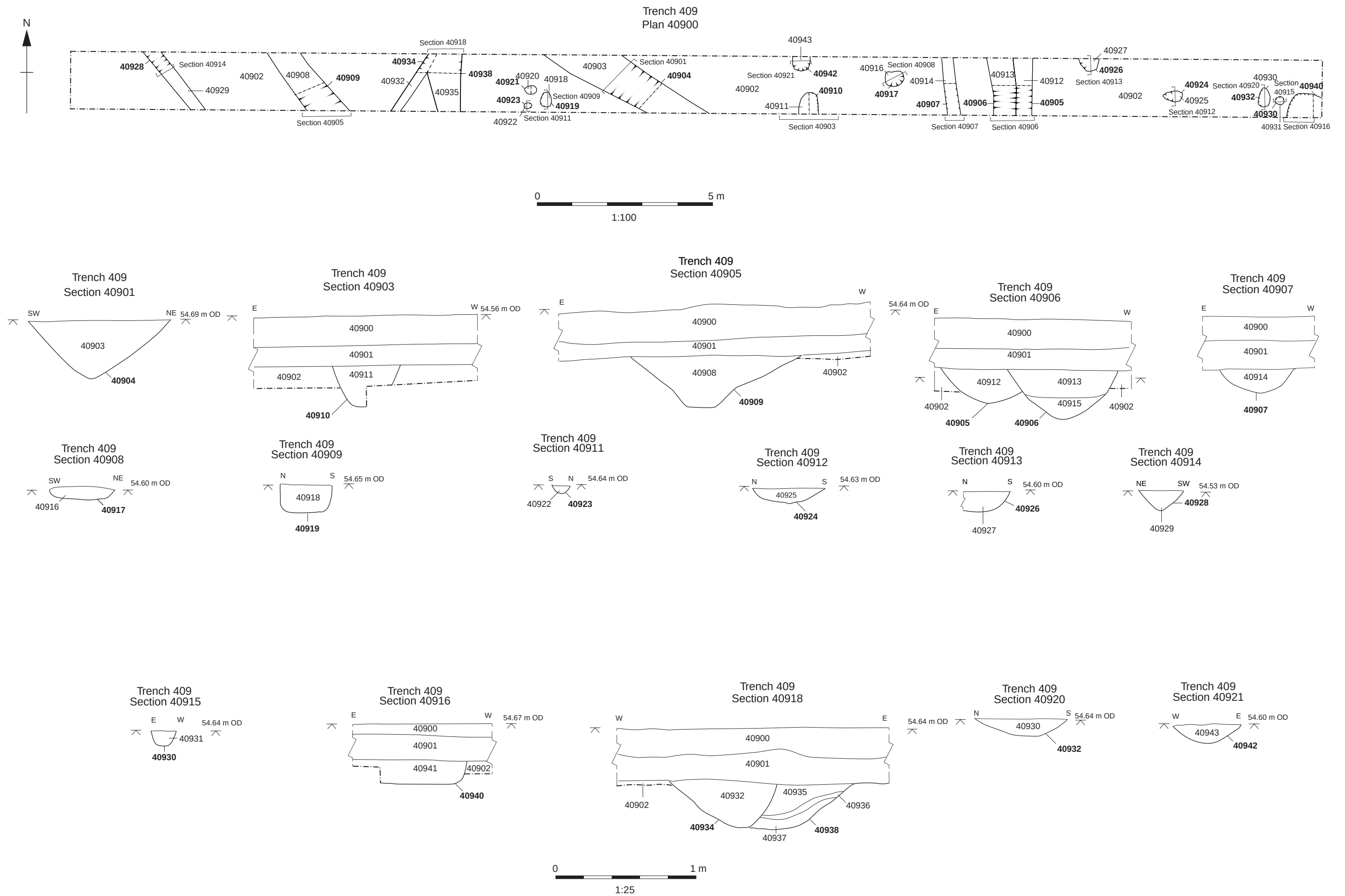
Figure 38: Area 3, Trench 409 plan and selected sections
