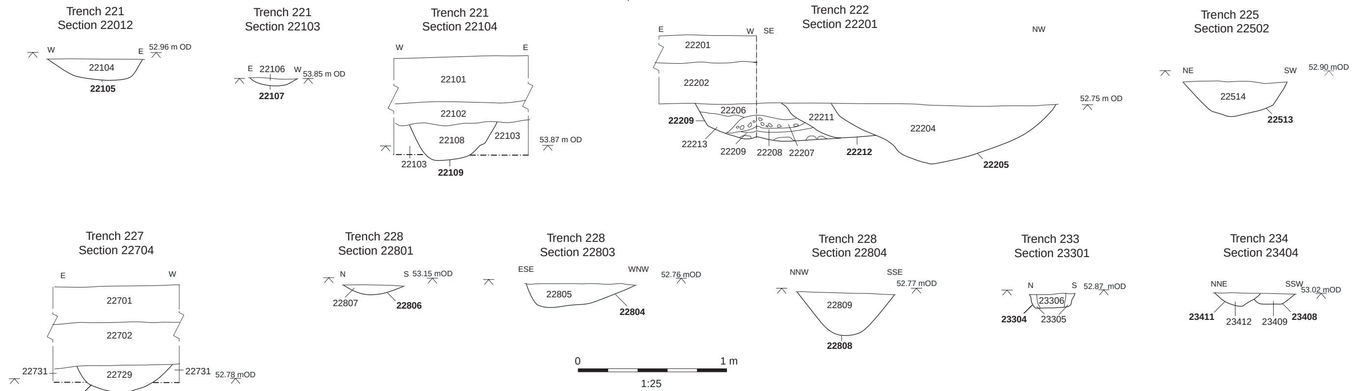
Figure 23: Field 4, Trench 231 plan and selected sections, Trenches 221, 222, 225, 227, 228, 233 and 234 selected sections
