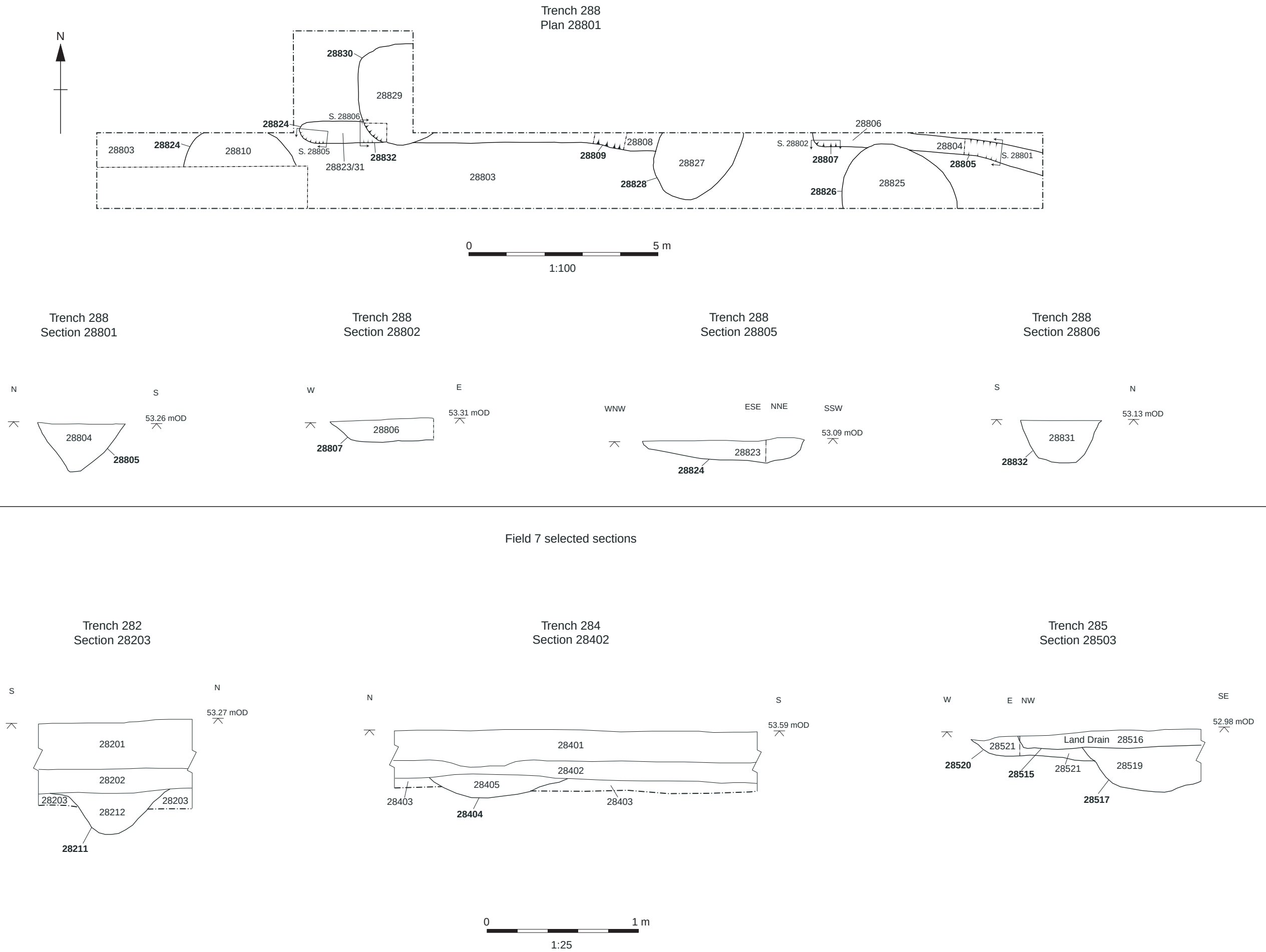
Figure 27: Field 7, Trench 288 plan and selected sections, Trenches 282, 284 and 285 selected sections
