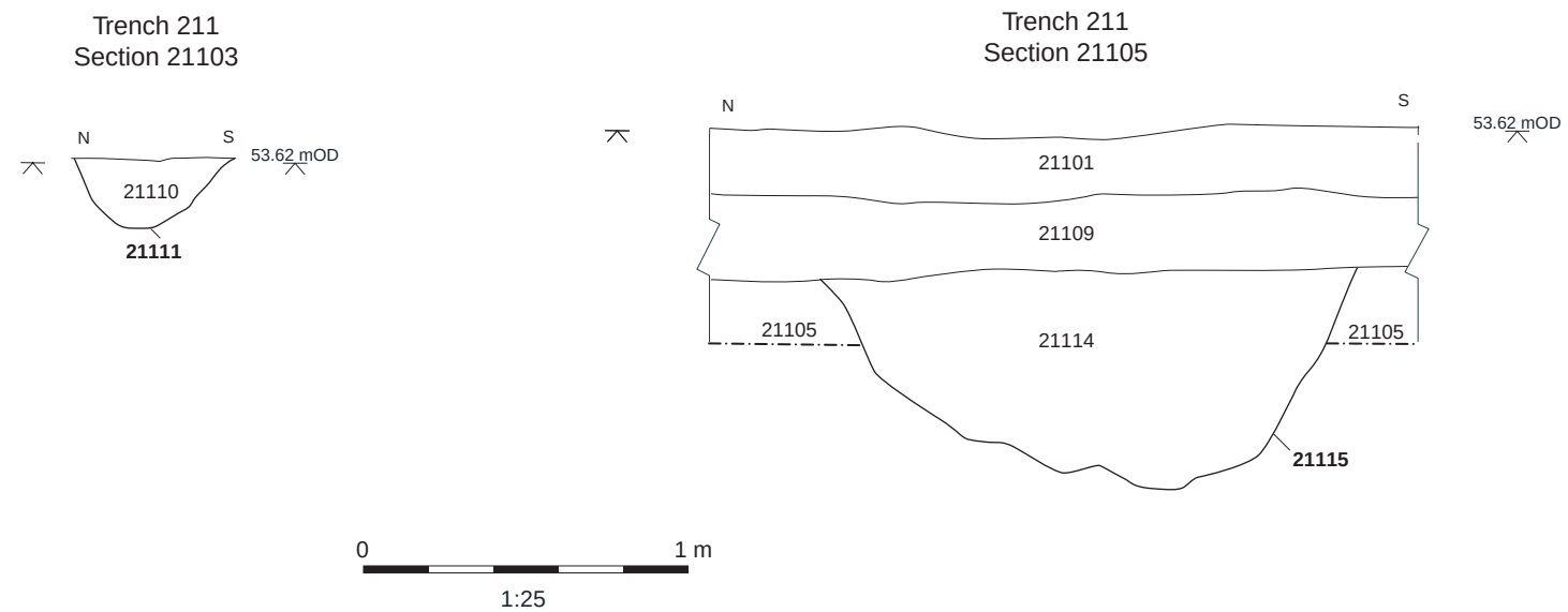
Figure 21: Field 4, Trench 212 plan and selected sections, Trench 211 selected sections
