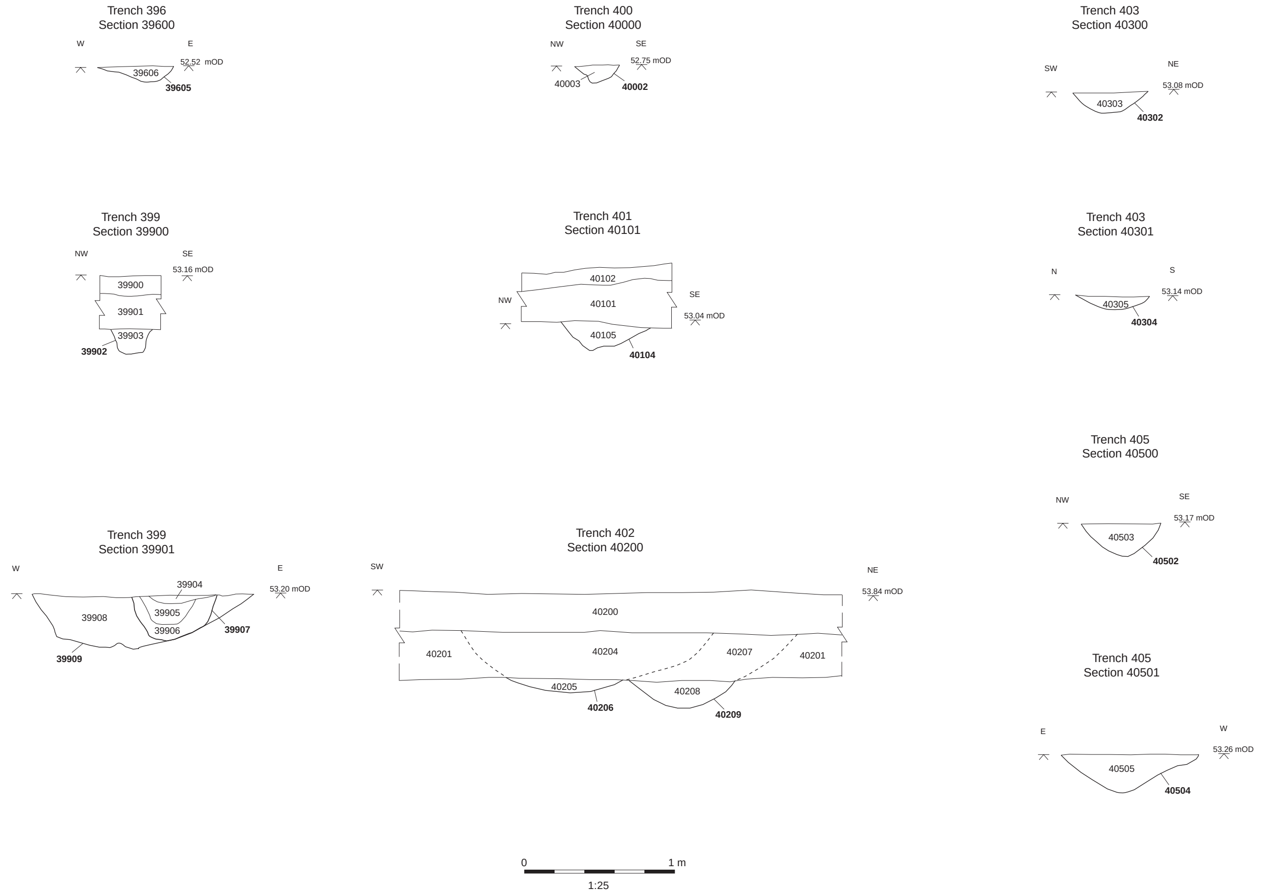
Figure 34: Areas 1 and 2, selected sections, Trenches 396, 399, 400, 401, 402, 403 and 405
